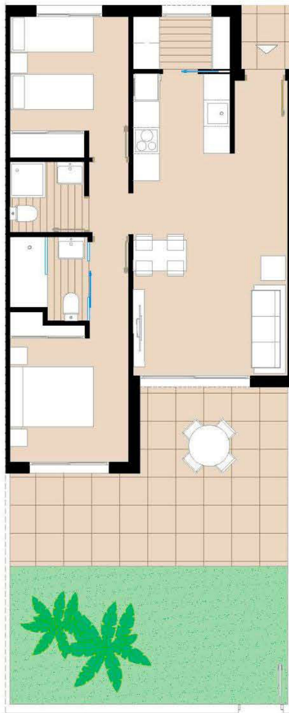
Ground Floor/ Planta Baja (E:1/100)
